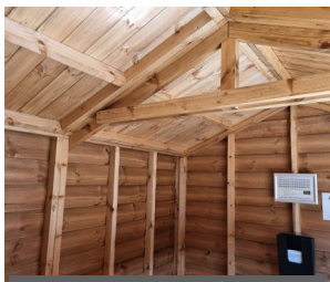
EX75MM X 50MM FRAMING
